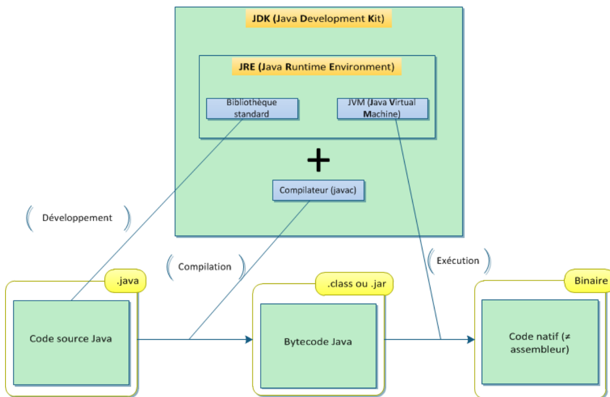
Figure 7.13 – Architecture Java
