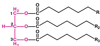
Triacyl-glycérol
